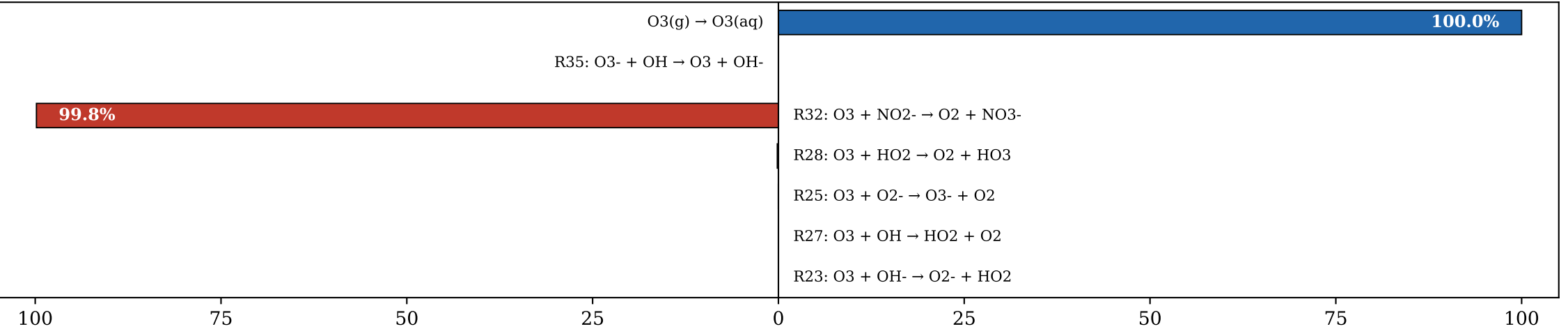
(c) NO 2 - (Σsrc = 8.44e-08 M/s)
